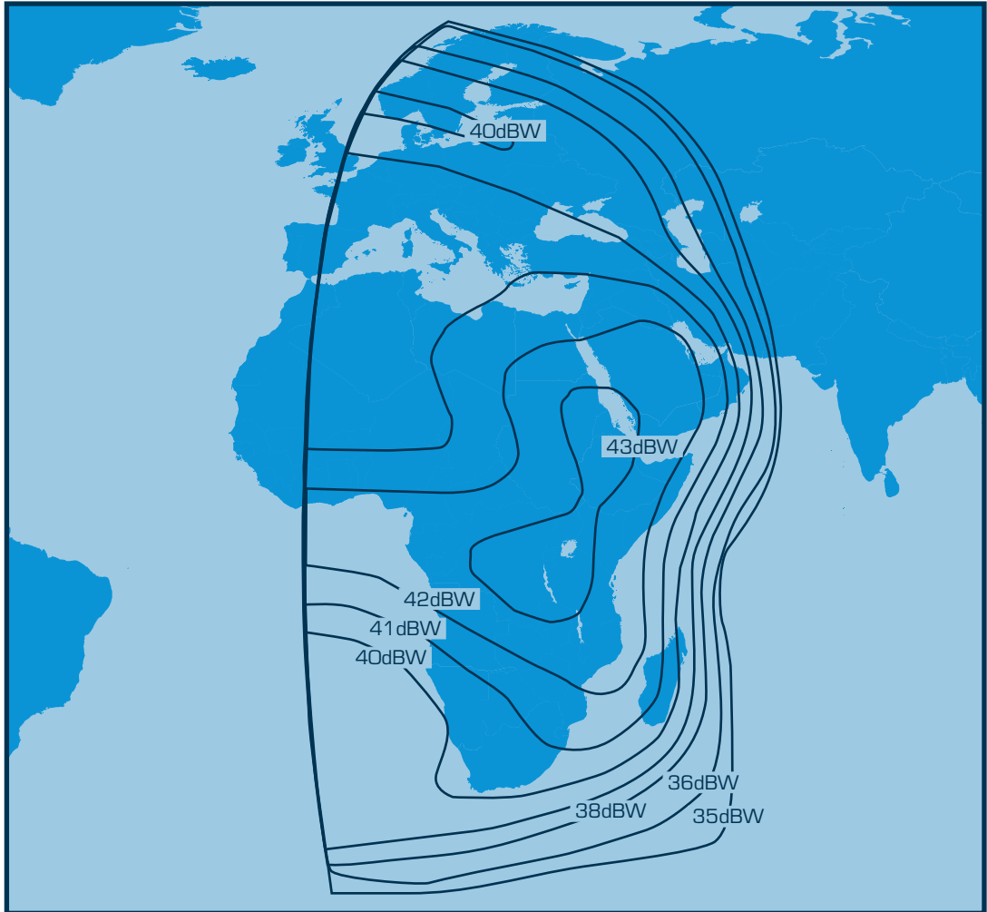
ABS-2, C-Band, West Hemi Beam, 75° East
